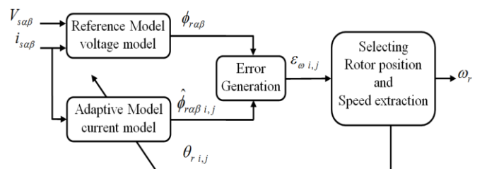
Fig. 3 The predictive MRAS speed observer
