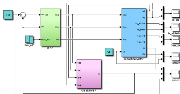
Fig. 5 Block diagram of sensorless induction motor drive with CMRAS/ PMRAS speed observers
