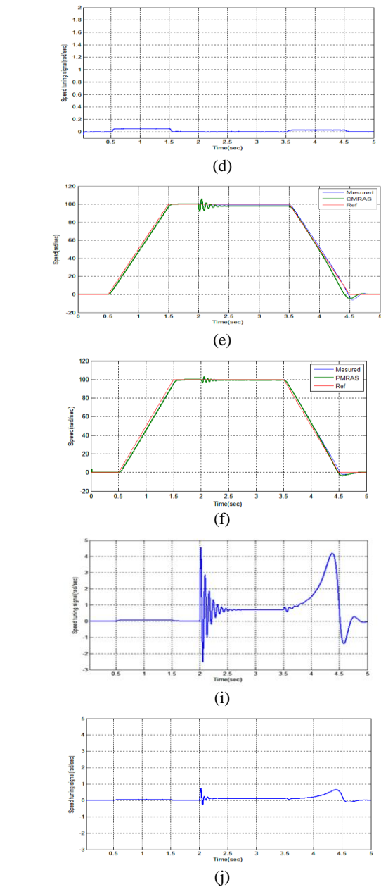
Fig. 8 simulation results of sensorless performance of induction motor drive with impact of rotor and stator resistances change. (a,e) rotor speed CMRAS, (b,f) rotor speed PMRAS, (c,i) speed error CMRAS, (d,j) speed error PMRAS.
