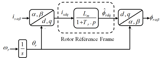
Fig. 2 The Adaptive model in the rotor reference frame
